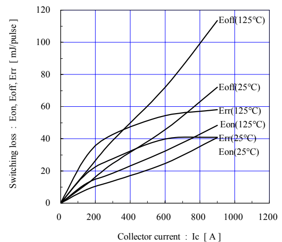
Switching loss vs. Collector current (typ.) V_{cc}=600V, V_{GE}=\pm 15V, R_g=0.6\Omega
