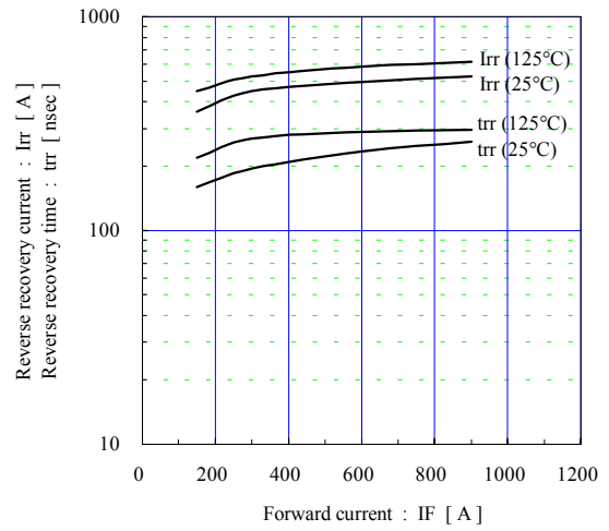
Reverse recovery characteristics (typ.) V_{cc}=600\text{V} , V_{GE}=\pm 15\text{V} , R_g=0.6\Omega
