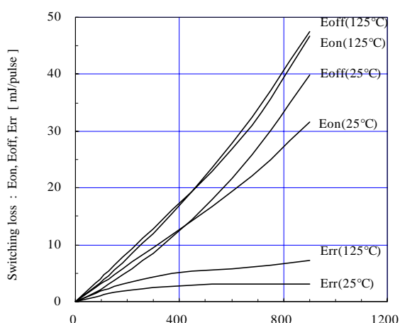
Switching loss vs. Collector current (typ.) V_{cc}=300V, V_{GE}=\pm 15V, R_g=4.7\Omega
