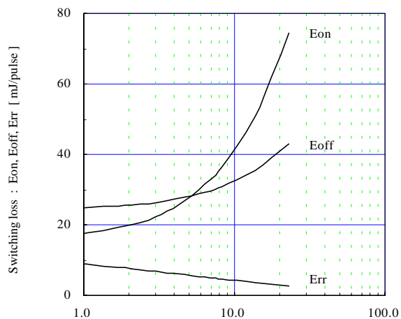
Switching loss vs. Gate resistance (typ.) V_{cc}=300V, I_c=600A, V_{GE}=\pm 15V, T_j=125^\circ C
