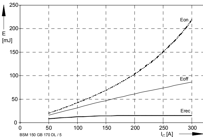
Bild / Fig. 5 Schaltverluste (typisch) / Switching losses (typical) E_{on} = f(I_C) , E_{off} = f(I_C) , E_{rec} = f(I_C) R_{g\text{on}} = R_{g\text{off}} = 10\Omega , V_{CE} = 900\text{V} , T_j = 125^\circ\text{C}
