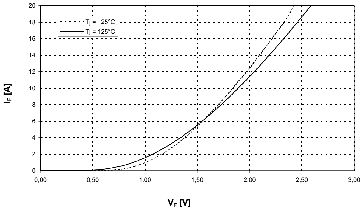
Forward characteristic of brake-chopper-FWD (typical)
