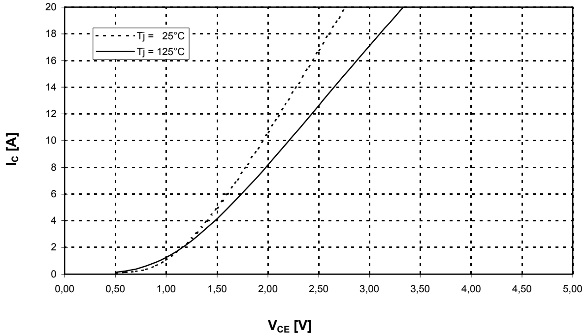
Output characteristic brake-chopper-IGBT (typical)
