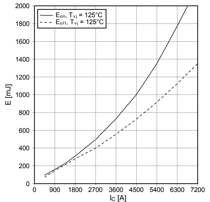
Schaltverluste IGBT-Wechselr. (typisch) switching losses IGBT-inverter (typical) E_{on} = f(I_c), E_{off} = f(I_c) V_{GE} = \pm 15\text{ V}, R_{Gon} = 0.8\ \Omega, R_{Goff} = 0.2\ \Omega, V_{CE} = 600\text{ V}
