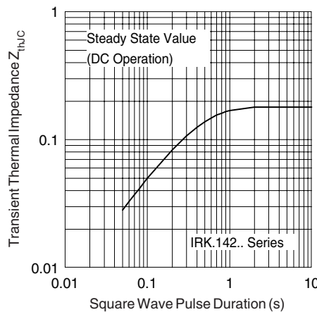
Fig.32 - Thermal Impedance Z_{thJC} Characteristics
